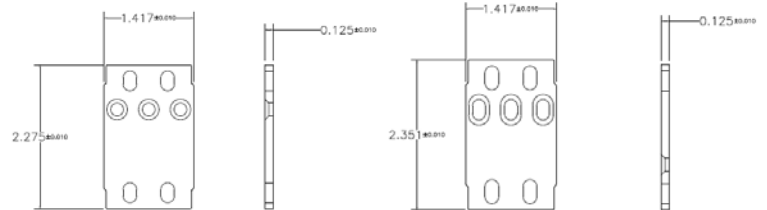
Level Bracket
